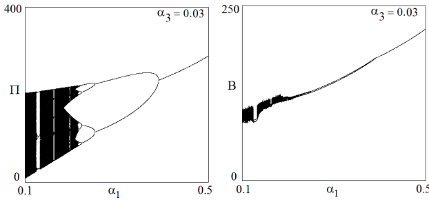
Fig. 3 One dimensional bifurcation diagrams. In (a) and (b) are shown the states of \Pi_t and B_t respectively, as \alpha_1 varies in the interval (0.1, 0.5) at \alpha_3 = 0.03 .
