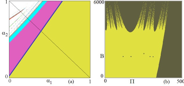
Fig. 5 In (a) Two-dimensional bifurcation diagram in the (\alpha_1, \alpha_2) parameter plane at i = -0.001 , \rho = 0.96 , a = 3.3 , b = 0.05 . In (b) dynamics in the phase space at the same parameters and \alpha_1 = 0.1 , \alpha_2 = 0.6 . The equilibrium is unstable and the attracting set is a cycle of period 4, its basin of attraction is in yellow. Gray points denote divergent trajectories.
