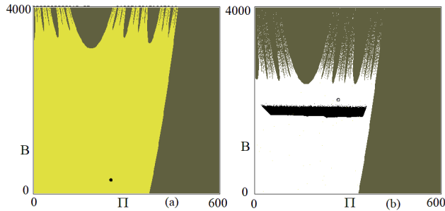
Fig. 2 The phase space in the case of positive net bonds ( \alpha_3 > 0 ). Phase space (II, B) represented at parameters as given in (14) and a = 3.3 . The gray region denotes points having a divergent trajectory. In (a) at (\alpha_1, \alpha_2) = (0.4, 0.55) (point A_1 in Figure 1) the fixed point is attracting and its basin of attraction is in yellow. In (b) at (\alpha_1, \alpha_2) = (0.1, 0.6) (point A_2 in Figure 1), the fixed point is unstable and a chaotic attractor, and the white points belong to its basin of attraction.
