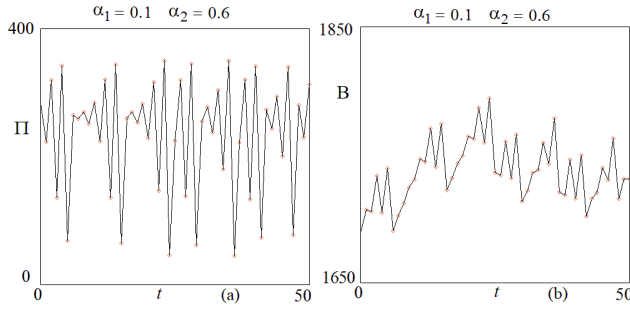
Fig. 4 Versus time trajectories. The parameters are fixed as in point A_2 in Figure 1 (a), at \alpha_1 = 0.1 and \alpha_2 = 0.6 , in a chaotic regime. Versus time trajectories of \Pi_t (in (a)) and B_t (in (b)) for 50 iterations.
