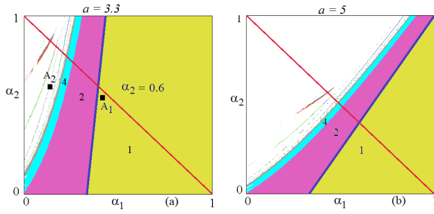
Fig. 1 Two dimensional bifurcation diagrams in the parameter plane (\alpha_1, \alpha_2) at fixed values given in (14) and a = 3.3 in (a), a = 5 in (b). The blue line is the bifurcation curve of equation \alpha_1 = \alpha_1^* given in (13). Below the diagonal of equation \alpha_1 + \alpha_2 = 1 it is \alpha_3 > 0 . The points A_1 and A_2 will be considered in Figure 2.
