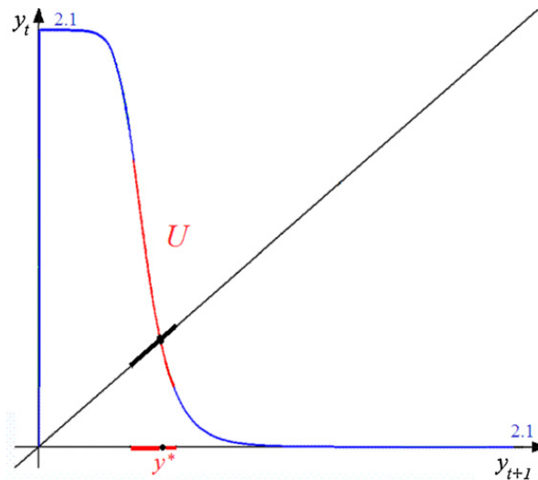
Fig. 7. Starting set U , neighborhood of y^* (in which |\chi'(x)| > 1 , for all x \in U ) of the function \chi at l^* = 2 , \alpha_1 = 0.5 and \alpha_2 = 14 .
