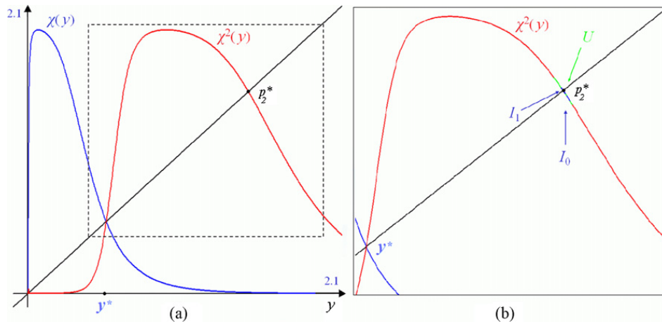
Fig. 9. In (a) graph of the function \chi at l^* = 2 , \alpha_1 = 0.5 and \alpha_2 = 8.22 , \alpha_2^\infty < \alpha_2 < \hat{\alpha}_2 and the graph of the second iterate of the function, \chi^2 . In (b) an enlargement of \chi^2 showing a point of the 2-cycle which is a snap-back repeller.
