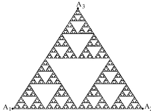
Fig. 3. Sierpinski triangle, unique attractor of the IFS \{D; H_1, H_2, H_3\} .
