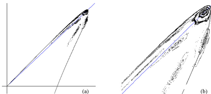
Fig. 13. Example of a forward equilibrium trajectory. In (a) a trajectory of the RIFS similar to the “chaos game” associated with the two-dimensional model, at a = 3 , l^* = 2 , \delta = 0.2 , \alpha_1 = 0.5 and \alpha_2 = 2.45 . The portion of phase plane (q, r) is [0.3, 0.65] \times [0.3, 0.65] . In (b) an enlargement of (a) is shown.
