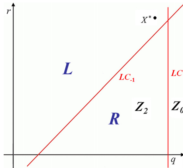
Fig. 10. Two-dimensional phase plane separated in two regions ( R and L ) by the critical line LC_{-1} . Each point on the right of the line LC = T(LC_{-1}) , region Z_0 , has no rank-1 preimages, while each point on the left of the line LC , region Z_2 , has two distinct rank-1 preimages, one in R and one in L .
