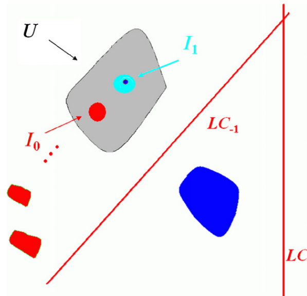
Fig. 11. Qualitative description of the neighborhood U involved in the construction of the sets I_0 = F(U) = T_{RL\dots L}^{-8}(U) \subset U and I_1 = G(U) = T_L^{-8}(U) \subset U . X^* \in I_1 .
