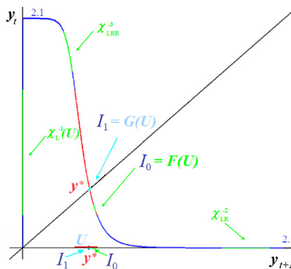
Fig. 8. A building up of the two disjoint intervals I_0 and I_1 belonging to U , for the function \chi at l^* = 2 , \alpha_1 = 0.5 and \alpha_2 = 14 . y^* \in I_1 .
