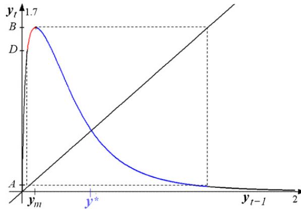
Fig. 5. Graph of the one-dimensional function \chi at l^* = 2 , \alpha_1 = 0.5 and \alpha_2 = 6 . \chi_L is the branch on the left of the critical point y_m with inverse \chi_L^{-1} , \chi_R is the branch on the right of y_m with inverse \chi_R^{-1} . The interval of interest is I = [A, B] = [A, D] \cup [D, B] , where B = \chi(y_m) , A = \chi^2(y_m) , D = \chi^3(y_m) .
